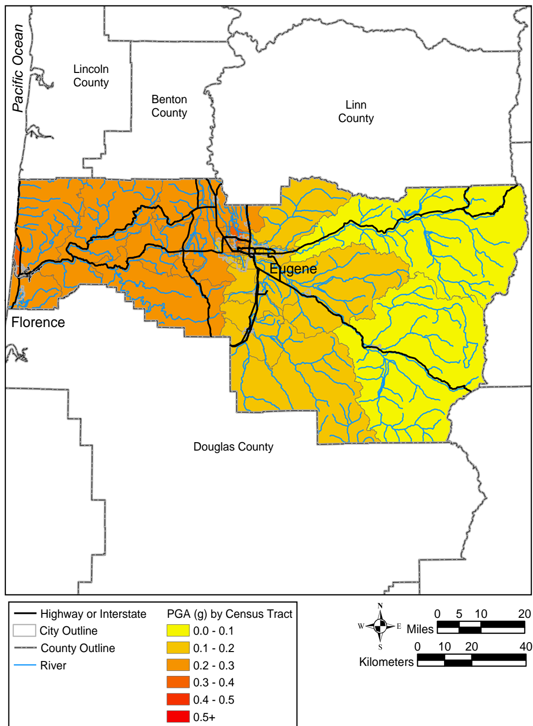
Figure C4. Peak ground acceleration (PGA) by census tracts map for the Cascadia Subduction Zone earthquake scenario, Lane County, Oregon (FEMA, 2003b).
