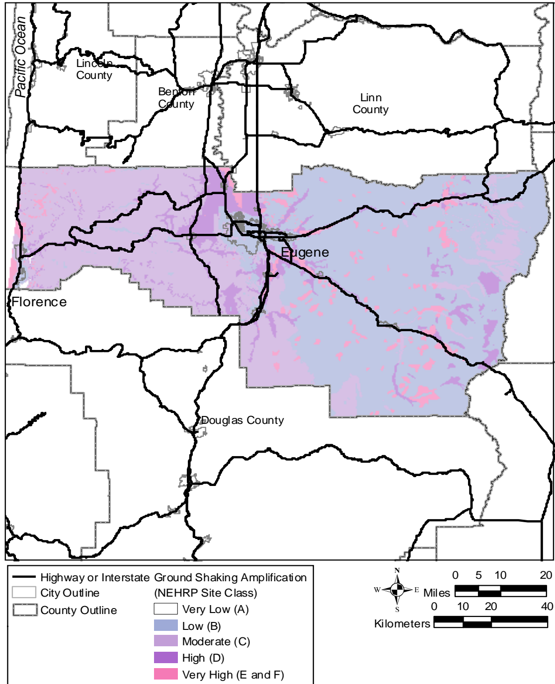
Figure C5. Relative ground-shaking amplification susceptibility map for Lane County, Oregon.
