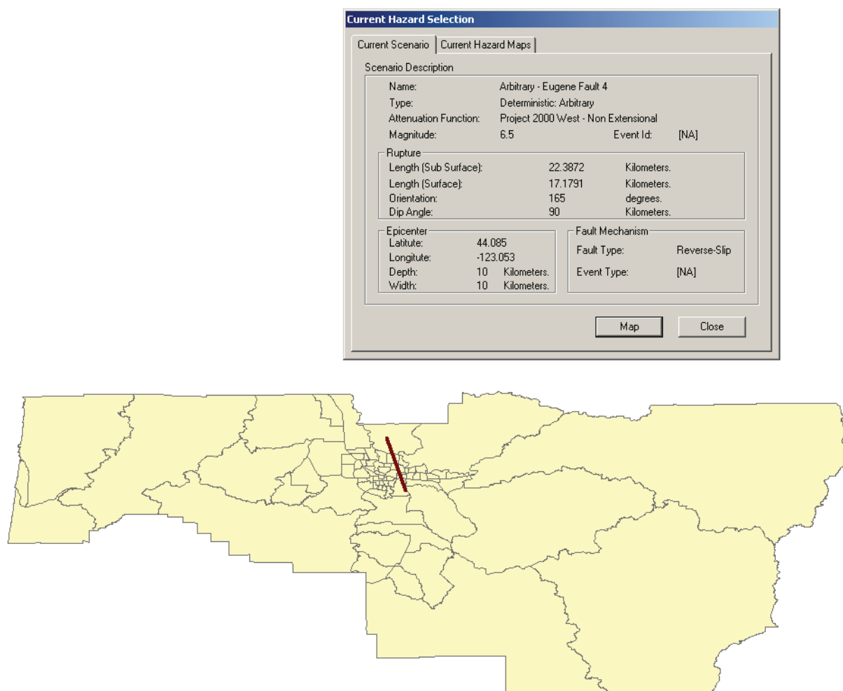
Figure C1. Arbitrary Eugene Fault details from HAZUS-MH (FEMA, 2003b). The location of the fault is shown as the dark line.
