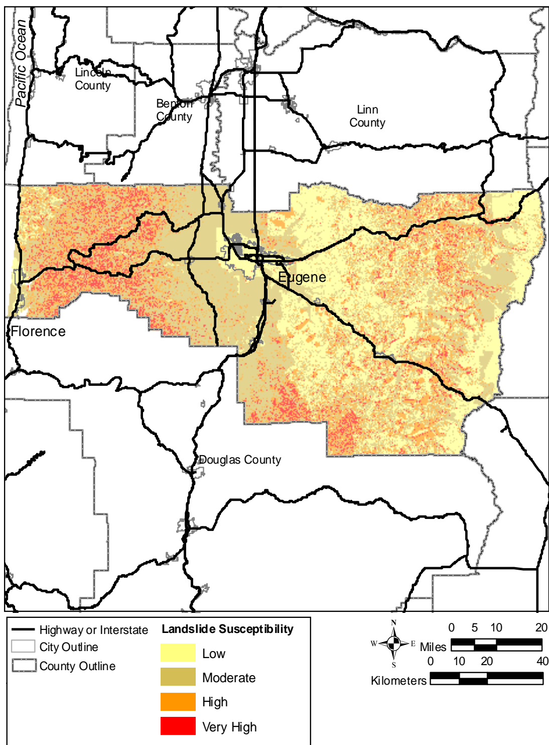
Figure C7. Relative earthquake-induced landslide susceptibility map for Lane County, Oregon.
