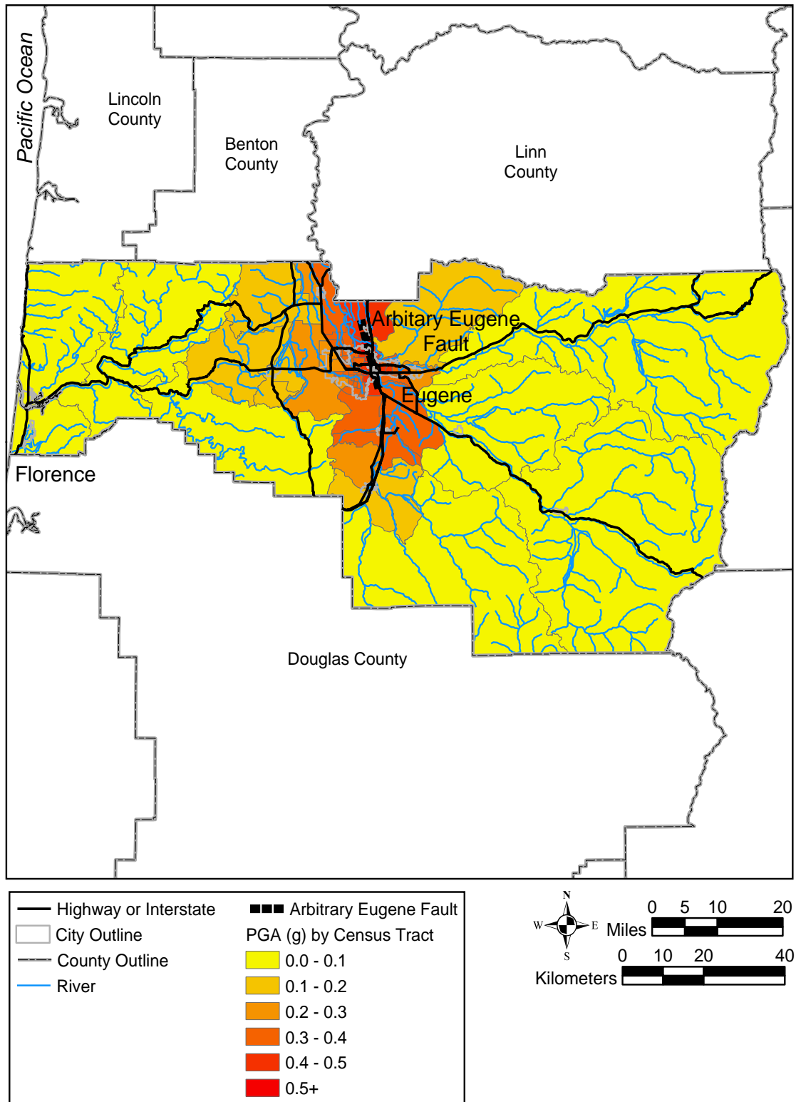
Figure C2. Peak ground acceleration (PGA) by census tracts map for the crustal earthquake scenario, Lane County, Oregon (FEMA, 2003b).
