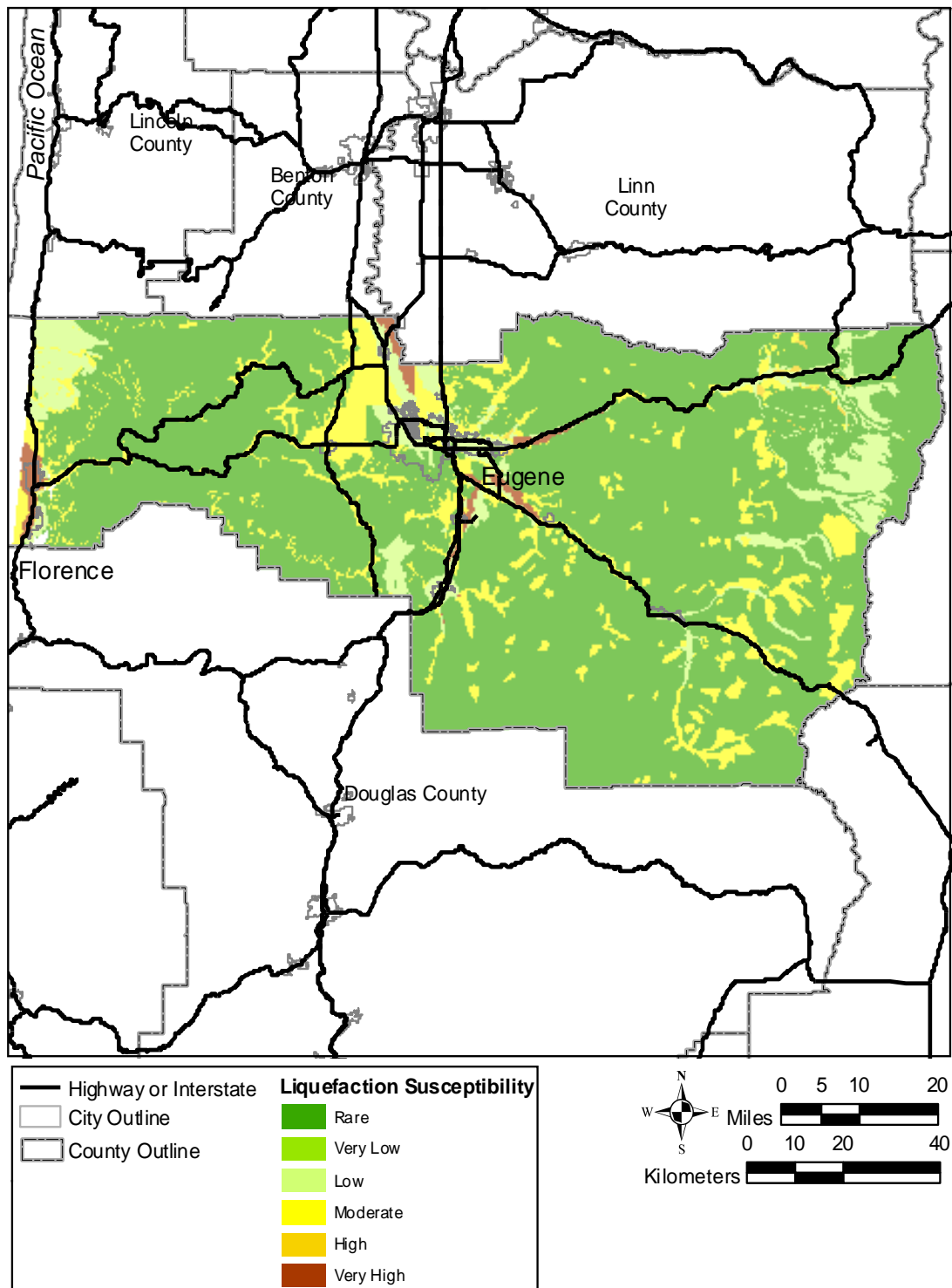
Figure C6. Relative liquefaction susceptibility map for Lane County, Oregon.
