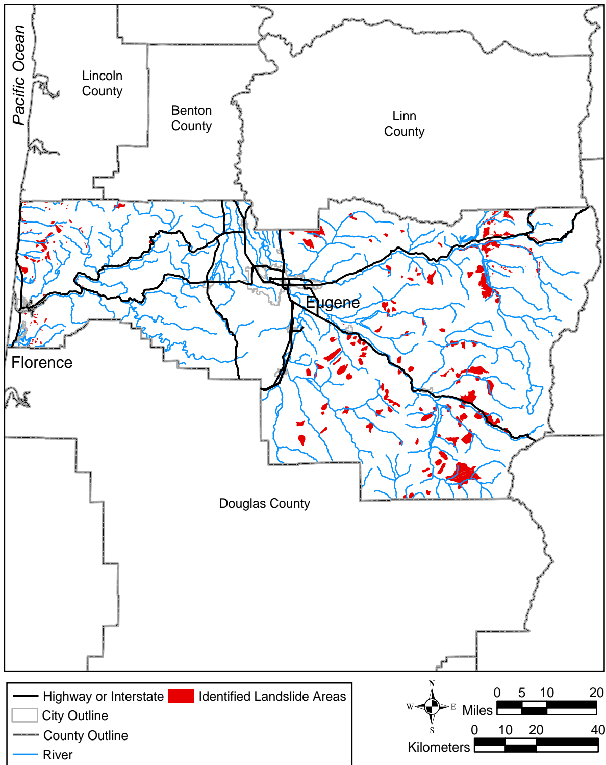
Figure C8. Identified landslide map for Lane County, Oregon.
