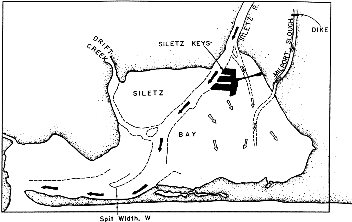
Figure 6. Circulation within Siletz Bay showing how erosion is focused on the thinnest part of the spit. Fills and dikes in the Siletz Keys-Milport Slough area aggravate the problem by preventing flood waters from spilling over into the south Bay. Figure from Komar and Rea (1976).
