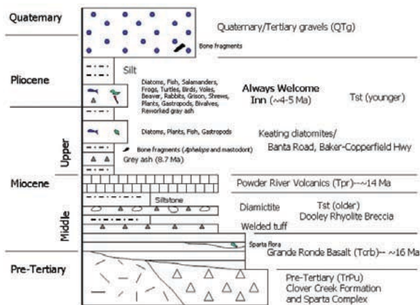
Figure 2. Generalized stratigraphy of the Tertiary sediments and volcanics of the study area. Modified from Ledgerwood and Van Tassell (2005).
