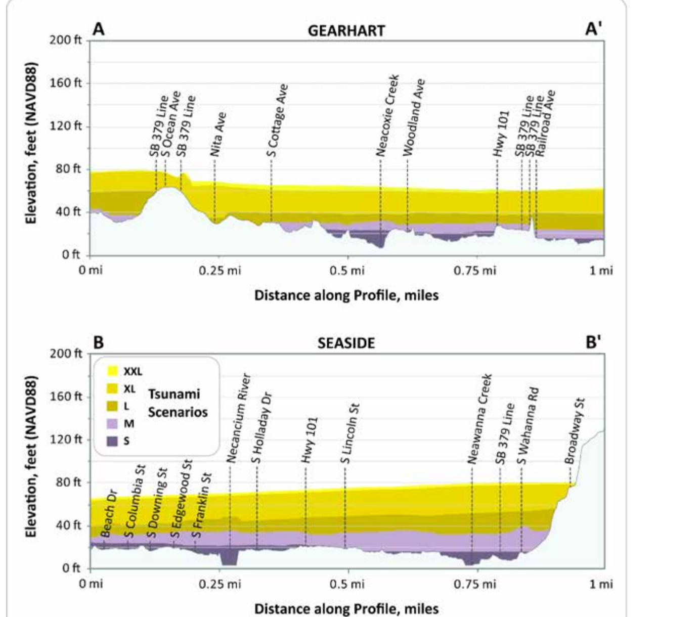
Figure 6: These profiles depict the expected maximum tsunami elevation for the five 'tsunami T-shirt scenarios' along lines A-A' and B-B'. The tsunami scenarios are modeled to occur at high tide and to account for local subsidence or uplift of the ground surface.
