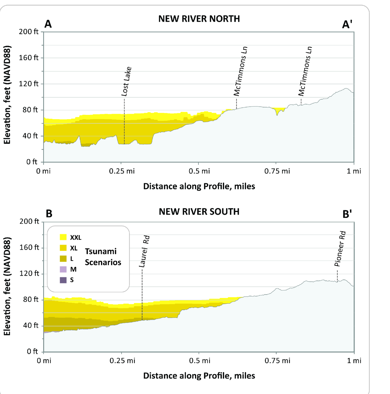
Figure 6: These profiles depict the expected maximum tsunami wave elevation for the five "tsunami T-shirt scenarios" along the New River. The tsunami scenarios are modeled to occur at high tide and to account for local subsidence or uplift of the ground surface.
