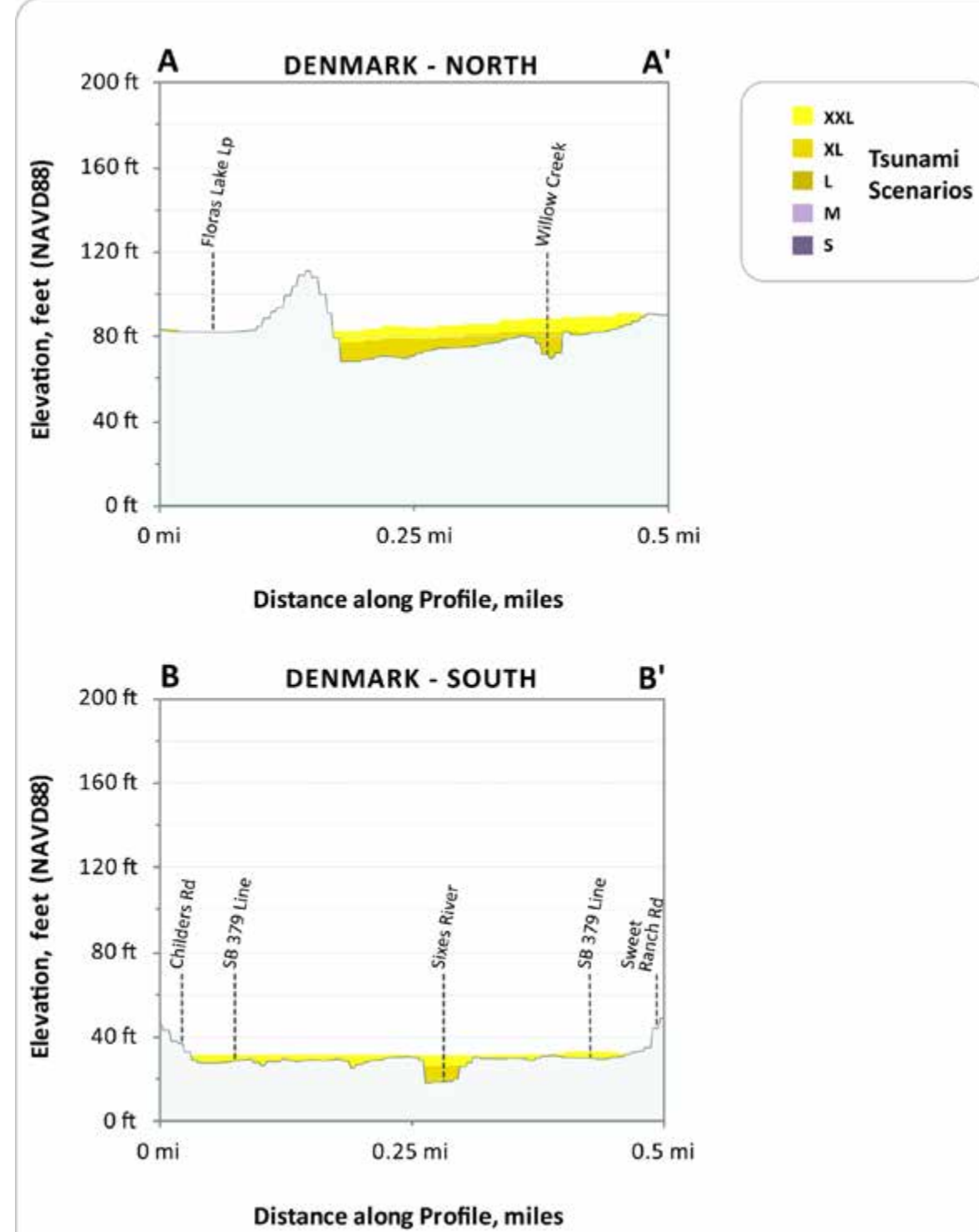
Figure 6: These profiles depict the expected maximum tsunami wave elevation for the five "Tsunami T-shirt scenarios" along lines A-A' and B-B'. The tsunami scenarios are modeled to occur at high tide and to account for local subsidence or uplift of the ground surface.
