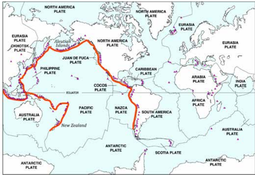
Figure 1: The "Ring of Fire" is a zone of active earthquakes and volcanoes that wraps much of the Pacific Ocean, including the Oregon coast. Volcanoes and earthquakes on this ring are caused by the movements of tectonic plates. One type of movement is called subduction - when thin, oceanic plates, such as those that compose the rock beneath the Pacific Ocean, sink beneath thicker, lighter plates that make up continental plates. Earthquakes that occur as a result of subduction can trigger tsunamis.
