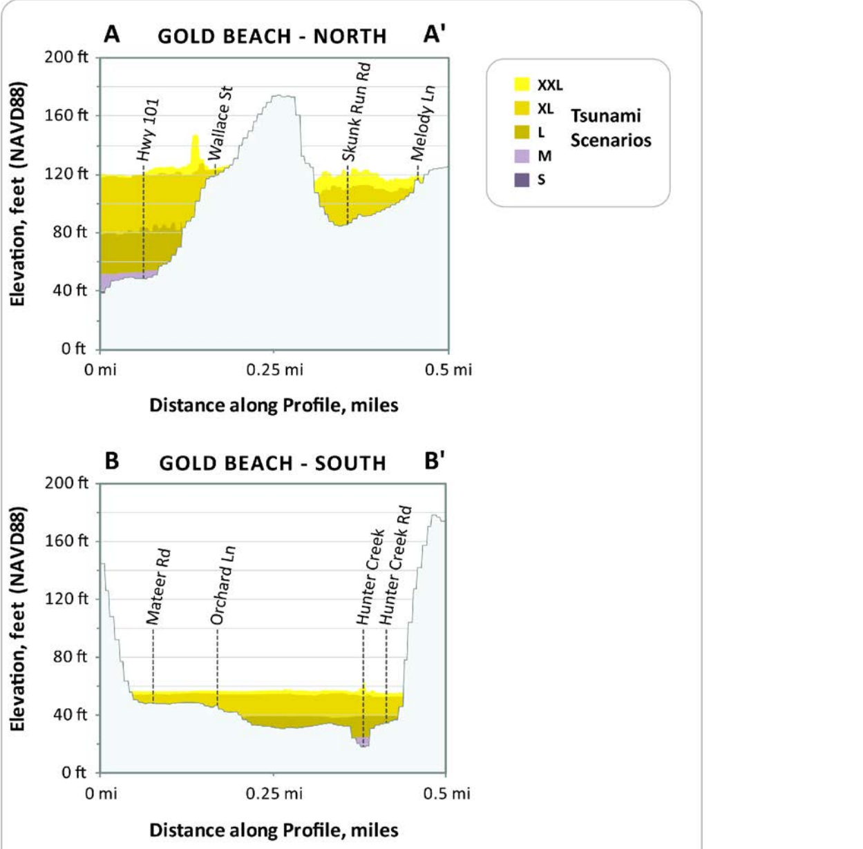
Figure 6: These profiles depict the expected maximum tsunami elevation for the five "T-shirt" scenarios along lines A-A' and B-B'. The tsunami scenarios are modeled to occur at high tide and to account for local subsidence or uplift of the ground surface.
