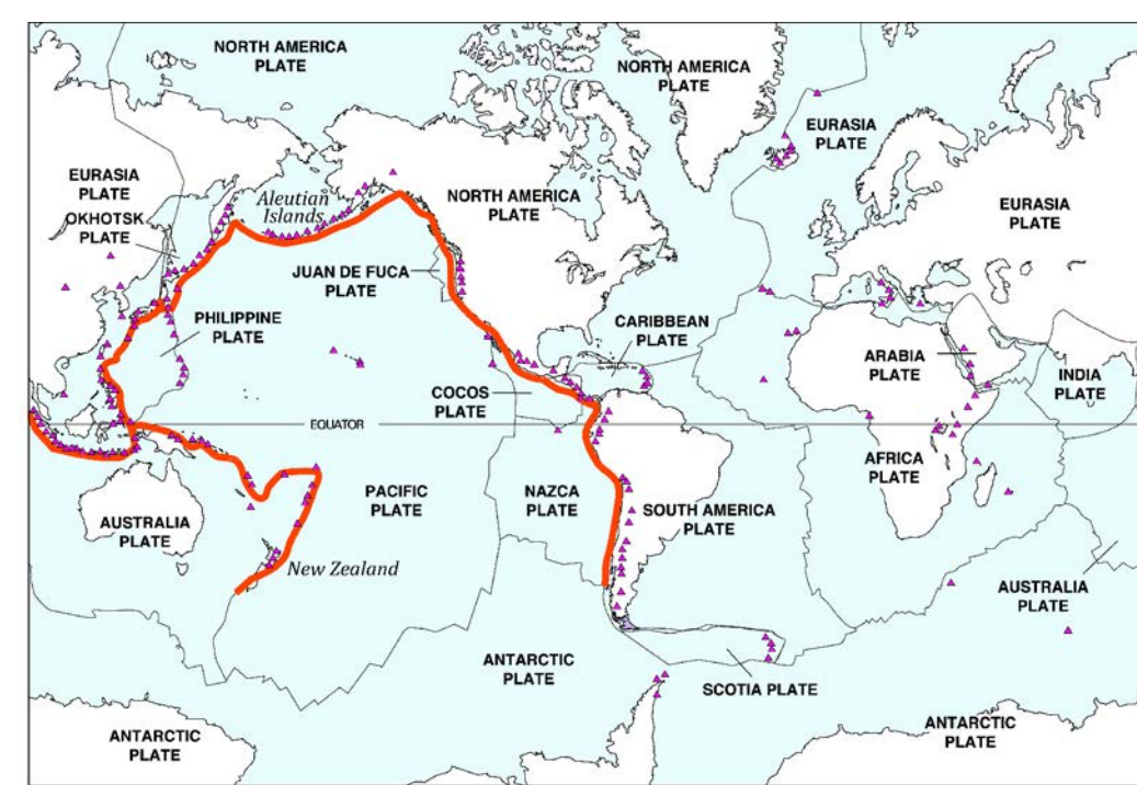
Figure 1: The "Ring of Fire" is a zone of earthquakes and volcanoes that rings much of the Pacific Ocean, including the Oregon coast. Volcanoes and earthquakes on this ring are caused by the movements of tectonic plates. One type of movement is called subduction - when thin, oceanic plates, such as those that compose the rock beneath the Pacific Ocean, sink beneath thicker, lighter plates that make up continental plates. Earthquakes that occur as a result of subduction can trigger tsunamis.
