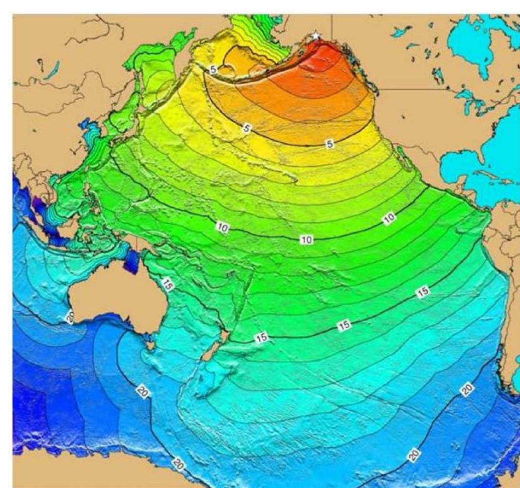
Figure 2: This image depicts the actual initial tsunami arrival times, in hours, around the Pacific Basin from the 1964 Prince William Sound earthquake. This magnitude 9.2 earthquake and resulting tsunami caused 125 deaths and $311 million in property loss, $84 million and 156 deaths in Alaska (NGDC/WHOI). The tsunami devastated many towns along the Gulf of Alaska, left serious damage in British Columbia, Hawaii, and along the west coast of the United States, and was recorded on tide gauges in Cuba and Puerto Rico.
