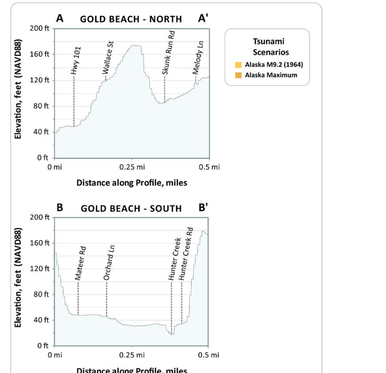
Figure 5: These profiles depict the expected maximum tsunami wave elevation for the two Alaska tsunami scenarios along lines A-A' and B-B'. The tsunami scenarios are modeled to occur at a static (no flow) tide and equal to the Mean Higher High Water (MHHW) high tide.
