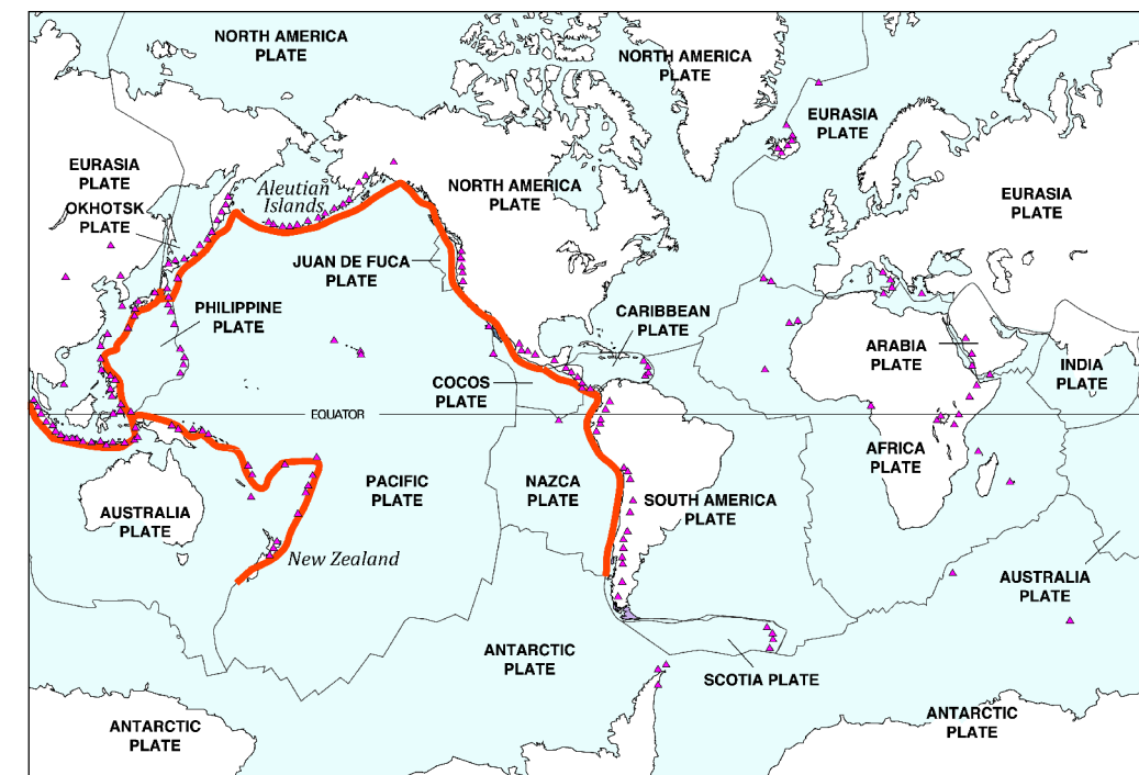
Figure 1: The "Ring of Fire" is a zone of earthquakes and volcanoes that rings much of the Pacific Ocean, including the Oregon coast. Volcanoes and earthquakes on this ring are caused by the movements of tectonic plates. One type of movement is called subduction - when thin, oceanic plates, such as those that compose the rock beneath the Pacific Ocean, sink beneath thicker, lighter plates that make up continental plates. Earthquakes that occur as a result of subduction can trigger tsunamis.
