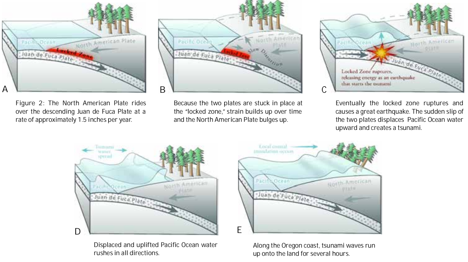
Figure 2. The North American Plate slips over the descending Juan de Fuca Plate at a rate of approximately 1.5 inches per year. Eventually the locked zone ruptures and causes a great earthquake. The sudden slip of the two plates displaces Pacific Ocean water upward and creates a tsunami. Displaced and uplifted Pacific Ocean water rushes in all directions. Along the Oregon coast, tsunami waves run up onto the land for several hours.
