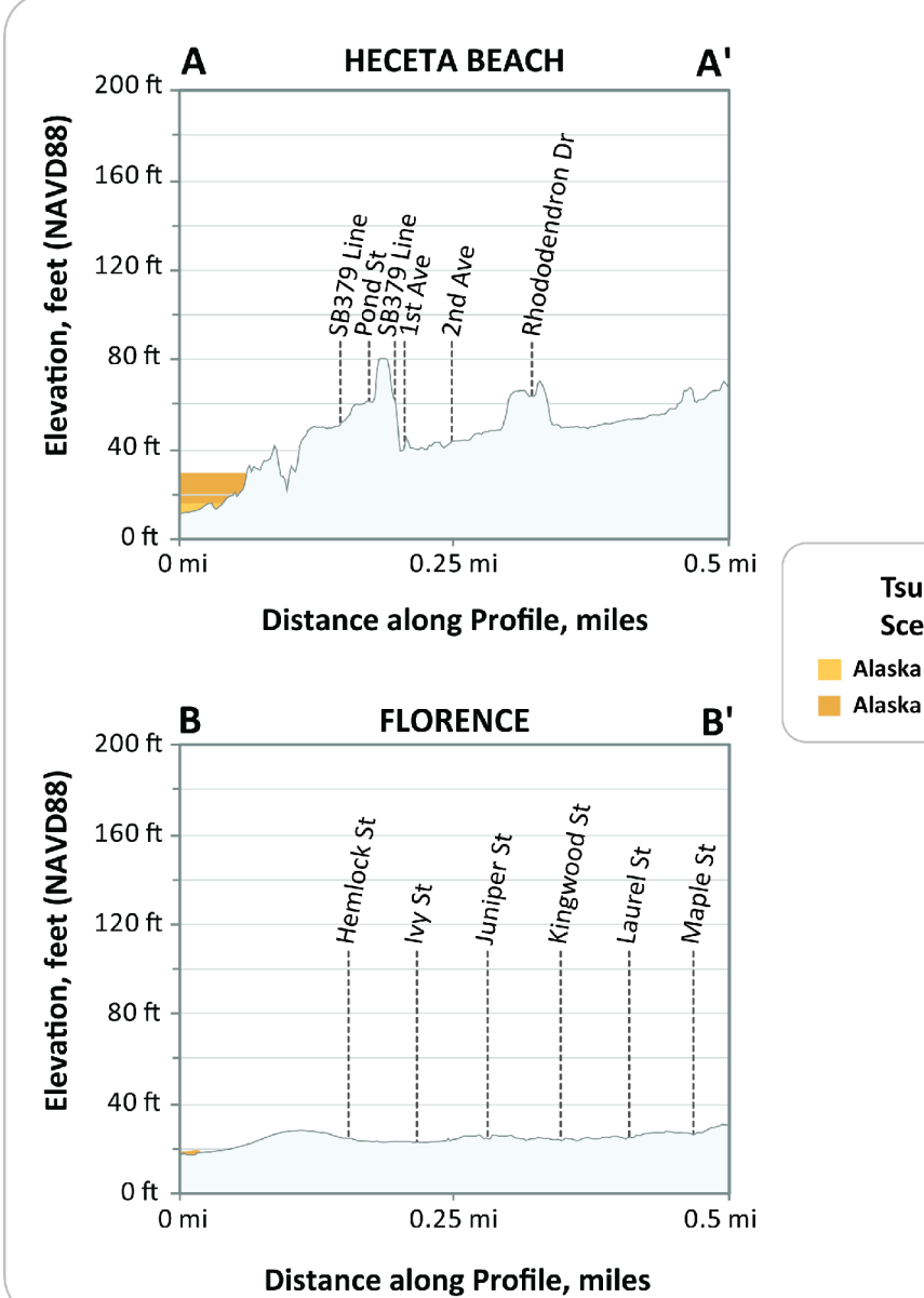
Figure 5: These profiles depict the expected maximum tsunami wave elevation for the two Alaska tsunami scenarios along lines A-A' and B-B'. The tsunami scenarios are modeled to occur at a static (on flow) tide and equal to the Mean Higher High Water (MHHW) high tide.
