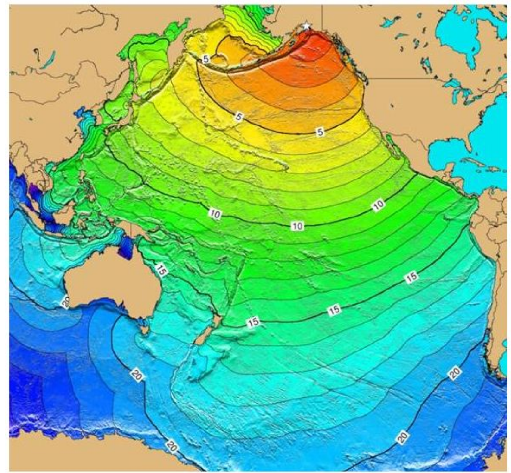
Figure 2: This map depicts the actual initial tsunami arrival times, in hours, around the Pacific Rim from the 1964 Prince William Sound earthquake. This magnitude 9.2 earthquake and resulting tsunami caused 175 deaths and $3.1 billion in property loss, 864 million and 106 deaths in Alaska (NOGS/NOCS). The tsunami devastated many towns along the Gulf of Alaska, left serious damage in British Columbia, Hawaii, and along the west coast of the United States, and was recorded on tide gauges in Cuba and Puerto Rico.
