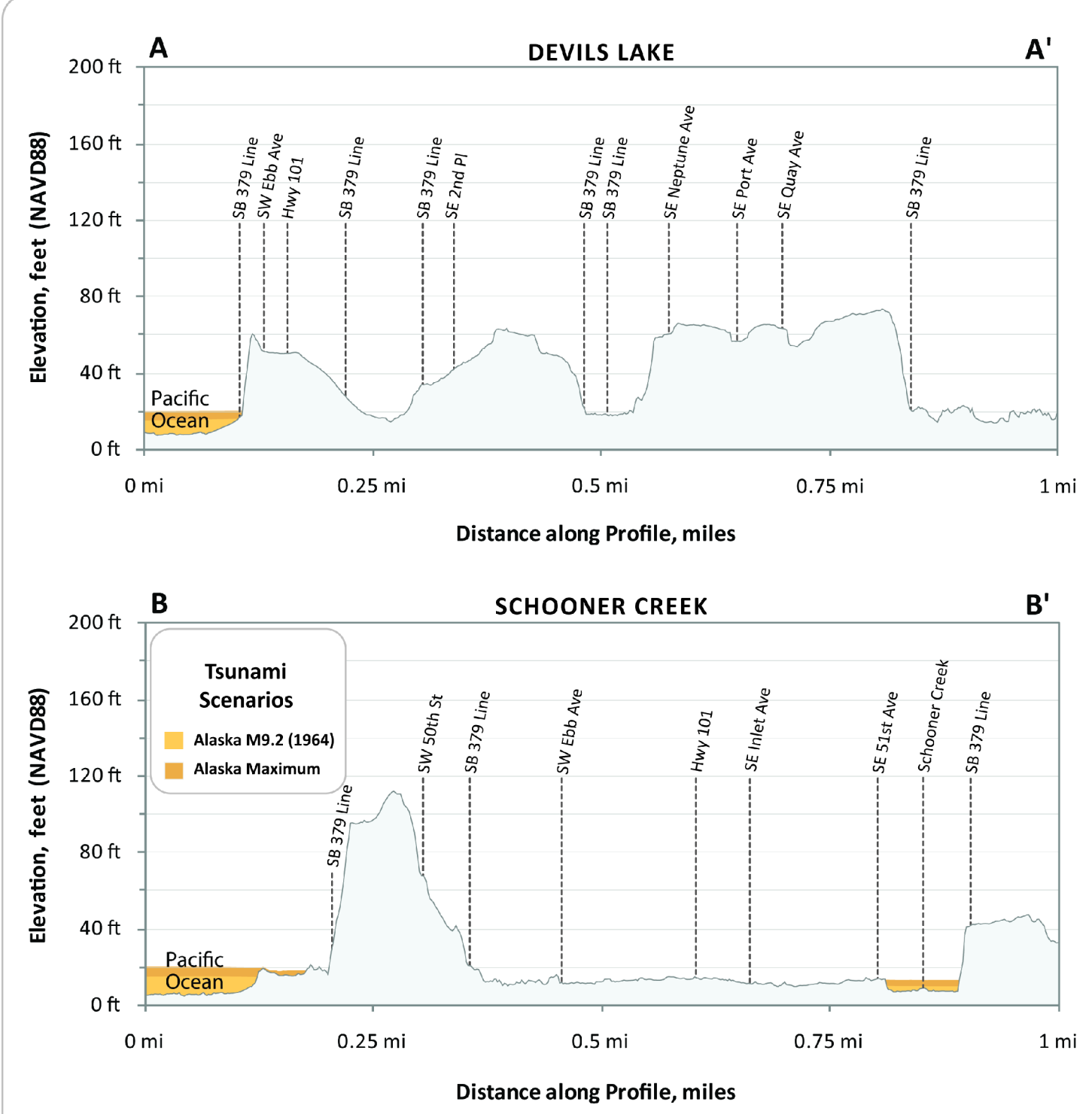
Figure 5. These profiles depict the expected maximum tsunami wave elevation for the two Alaska tsunami scenarios along lines A-A' and B-B'. The tsunami scenarios are modeled to occur at a static (no flow) tide and equal to the Mean Higher High Water (MHHW) high tide.
