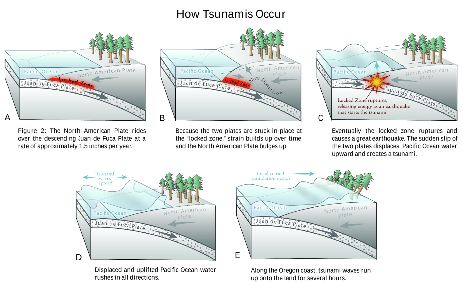
Figure 2: The North American Plate rides over the Juan de Fuca Plate at a rate of approximately 1.5 inches per year. Because the two plates are stuck in place at the "locked zone," strain builds up over time and the North American Plate bulges up. Eventually, the locked zone ruptures and causes a great earthquake. The sudden slip of the two plates displaces Pacific Ocean water upward and creates a tsunami.
