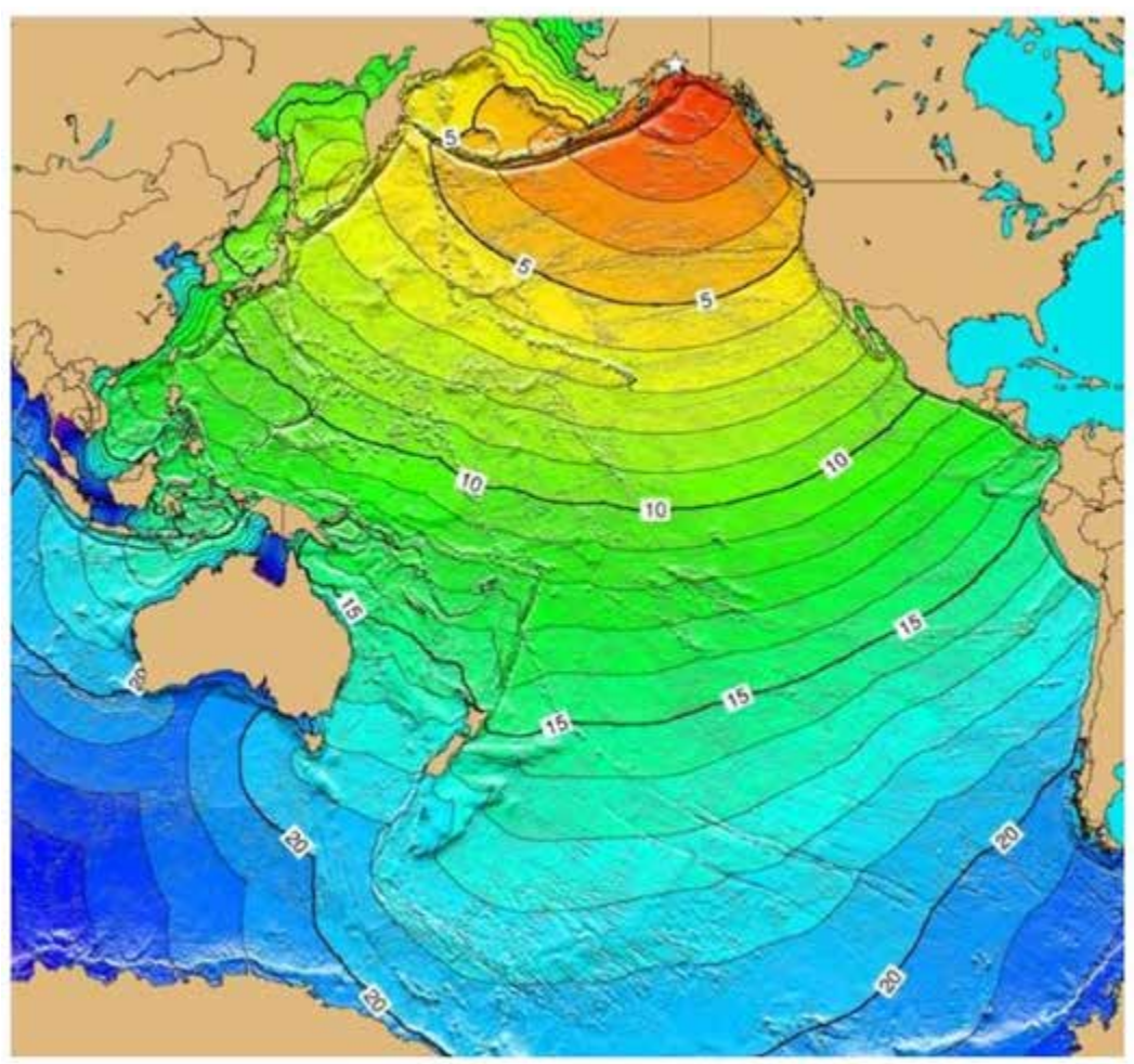
Figure 2: This image depicts the actual travel time of tsunami waves, in hours, around the Pacific Rim from the 1964 Prince William Sound earthquake. This magnitude 9.2 earthquake and resulting tsunami caused 125 deaths and $21.1 million in property loss in Alaska (NGDC/NOAA). The tsunami devastated many towns along the Gulf of Alaska, left serious damage in British Columbia, Hawaii, and along the west coast of the United States, and was recorded on tide gauges in Cuba and Puerto Rico.
