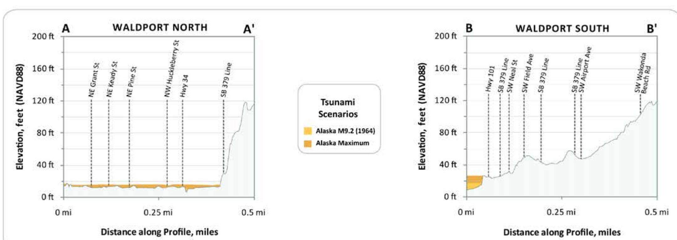
Figure 5: These profiles depict the expected maximum tsunami wave elevation for the two Alaska tsunami scenarios along lines A-A' and B-B'. The tsunami scenarios are modeled to occur at a slack (no flow) tide and equal to the Mean Higher High Water (MHHW) high tide.
