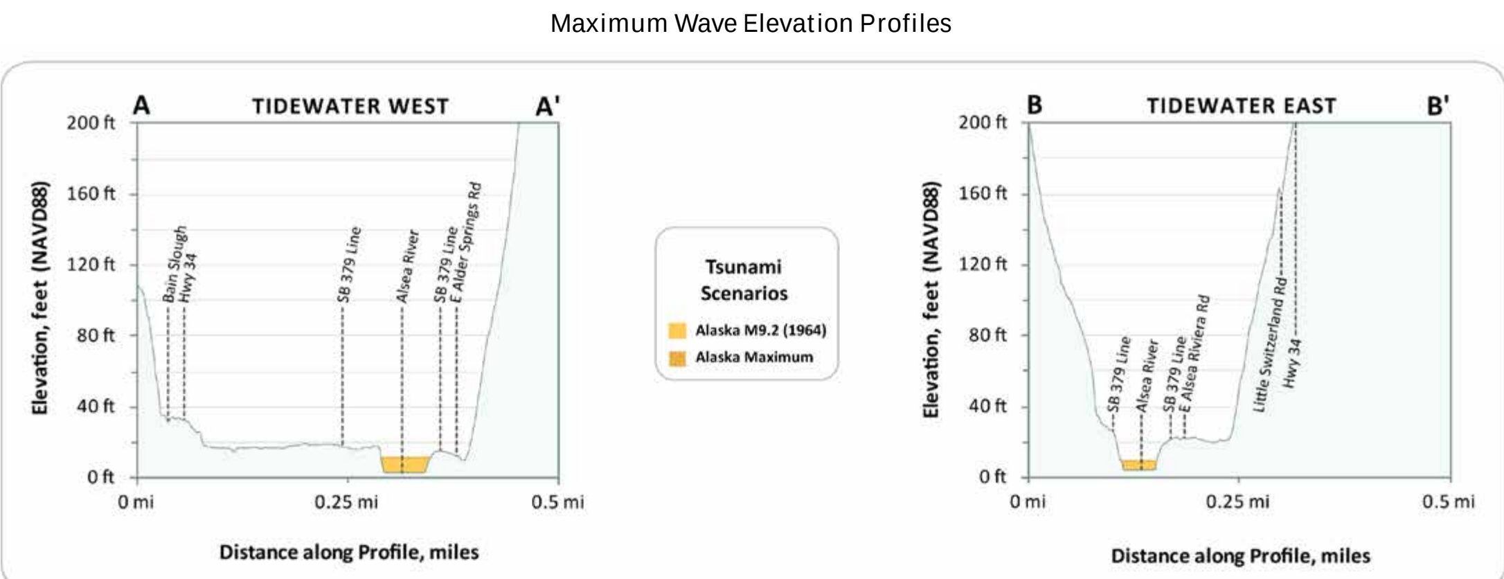
Figure 5. These profiles depict the expected maximum tsunami wave elevation for the two Alaska tsunami scenarios along lines A-A' and B-B'. The tsunami scenarios are modeled to occur at a static (no flow) tide and equal to the Mean Higher High Water (MHHW) high tide.
