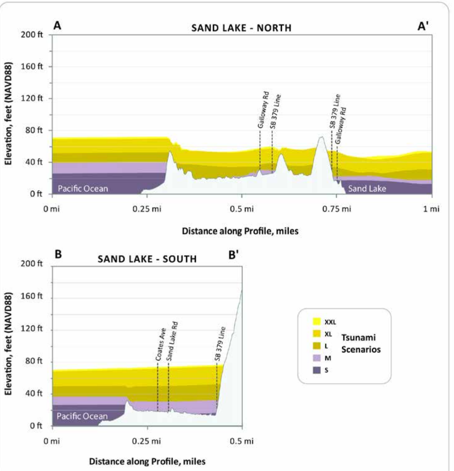
Figure 6: These profile graphs depict the expected maximum tsunami wave elevation for the five "T-shirt" scenarios along lines A-A' and B-B'. The tsunami corridors are modeled to occur at high tide and to account for local subsidence or uplift of the ground surface.
