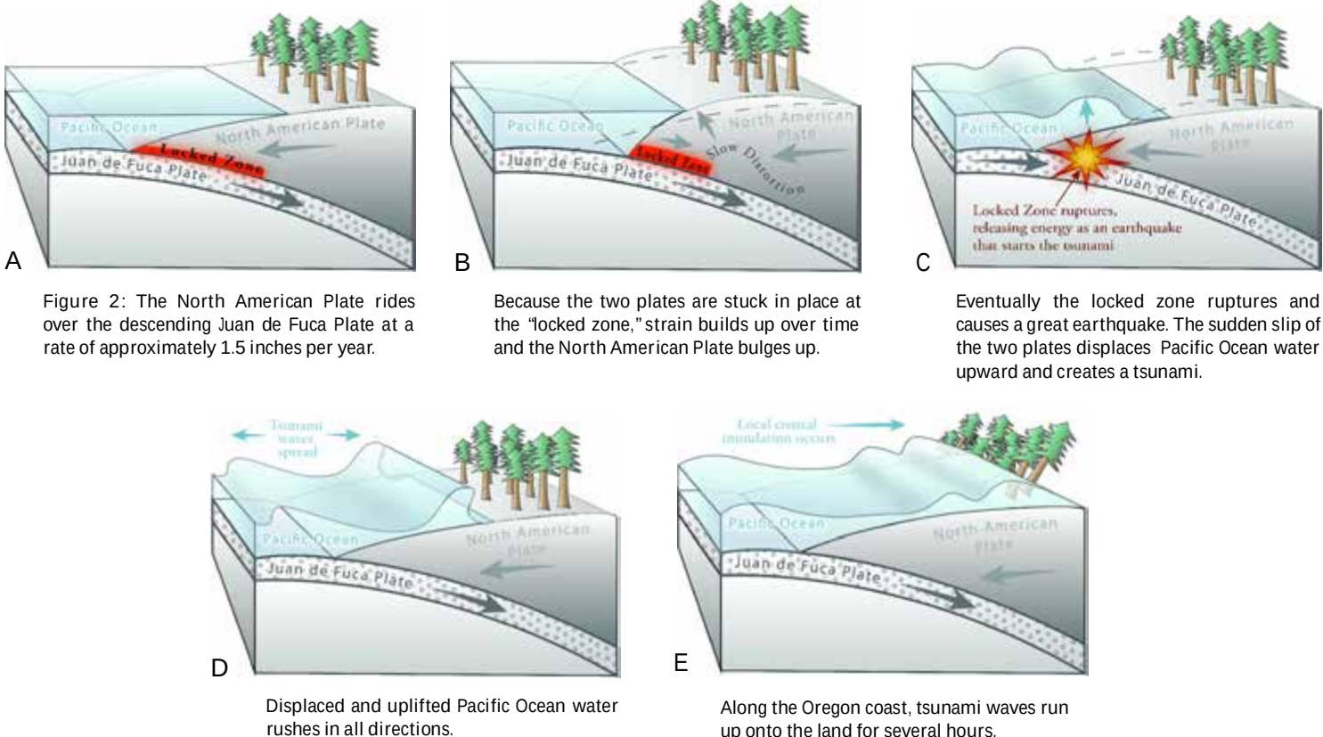
Figure 2: The North American Plate rides over the descending Juan de Fuca Plate at a rate of approximately 1.5 inches per year.
